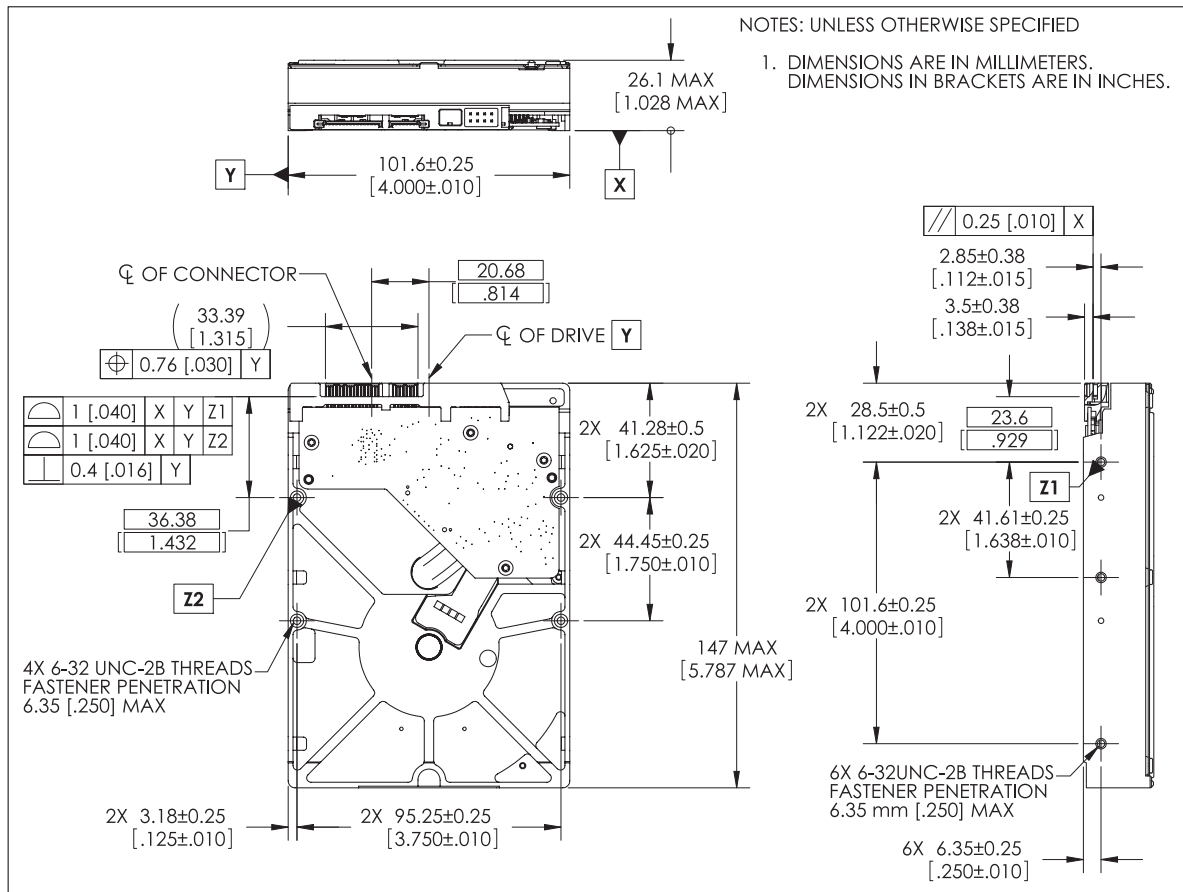
Figure 2-1. Mounting Dimensions
